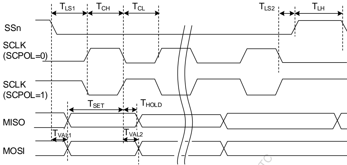
Figure 11. Motorola SPI Mode 1/3 (SCPH = 1)
