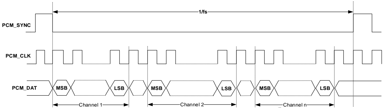
Figure 20. PCM short-frame timing diagram
