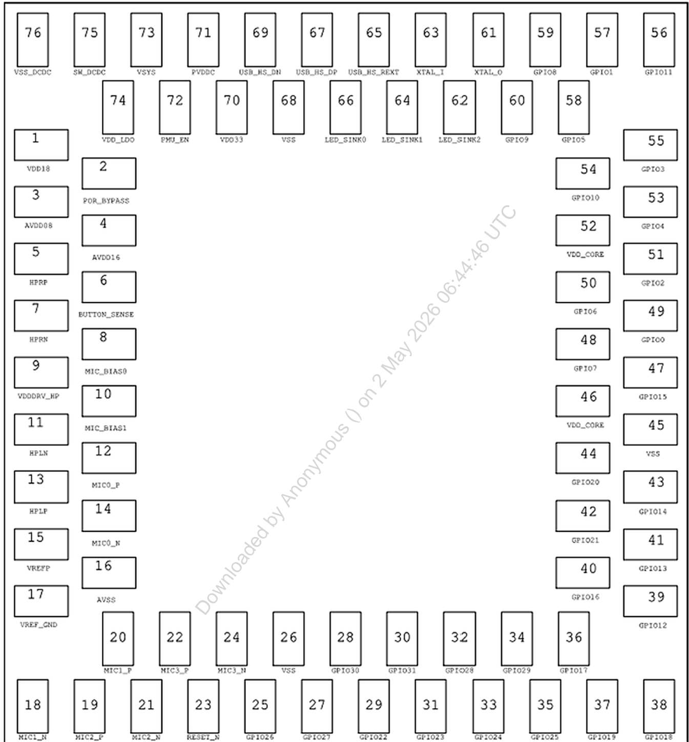
Figure 3. SR80 Series pin assignment (package pads facing down)
