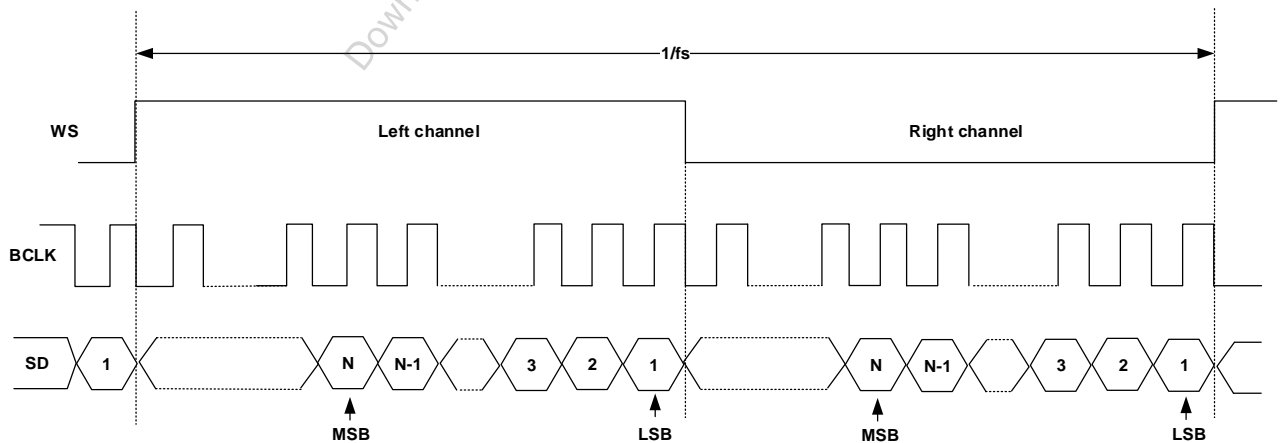
Figure 19. Right-justified timing diagram
