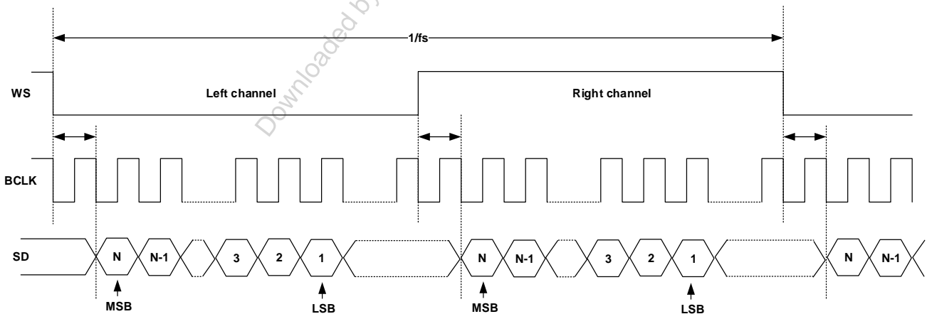
Figure 17. I2S timing diagram – width of LRCLK frame is wider than 2N bits (N = 8, 16, 24, or 32)
