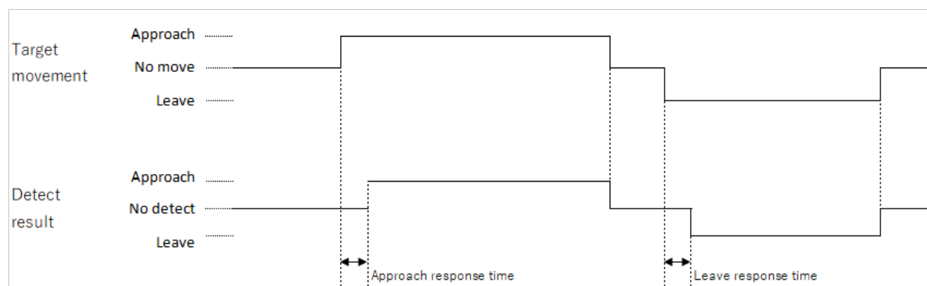
Fig. 20 Detection timing chart
