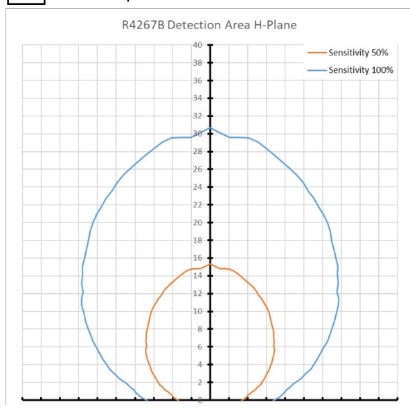
Fig. 12 B type H plane detection area
