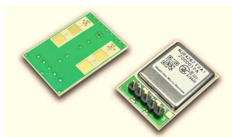
Outline : 17.2mm x 25mm x 3.1mm
