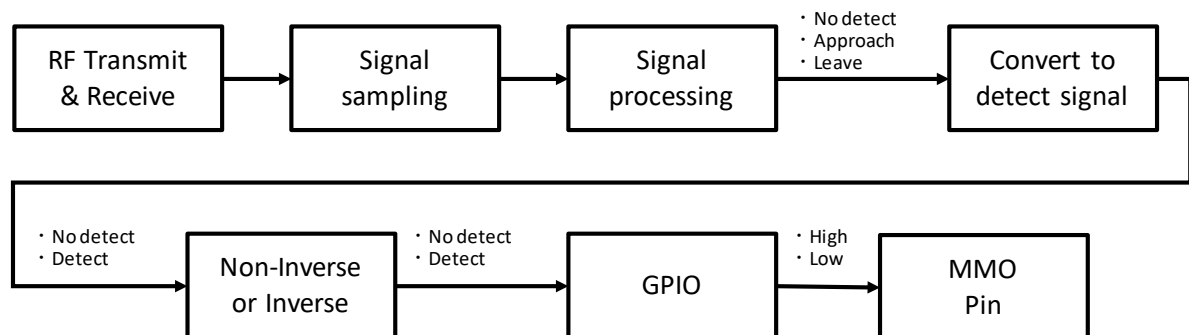
Fig. 14 Digital mode output flow chart
