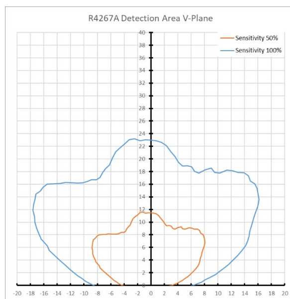
Fig. 11 A type V plane detection area
