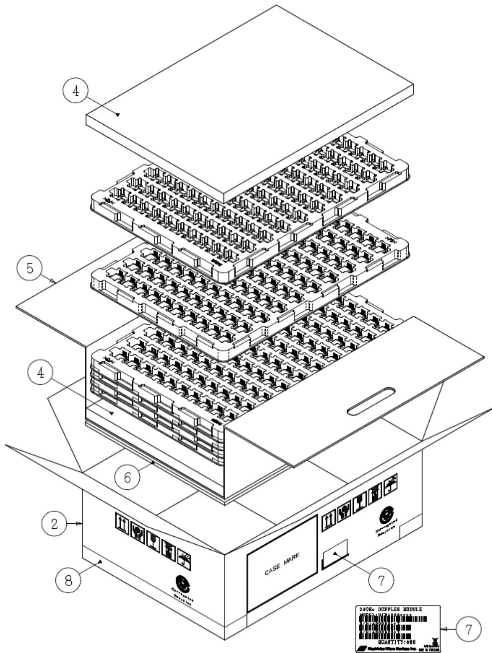
Fig. 37 Packing Diagram
