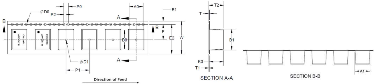
Tape Dimension(mm)
