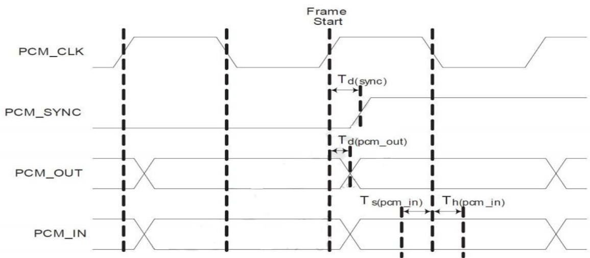
PCM interface timing diagram (slave)
