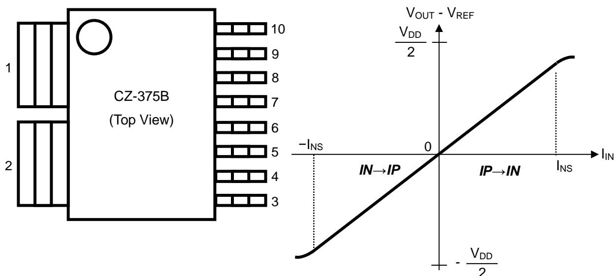
Figure 2. Pin configurations and typical output characteristics of CZ-375B
