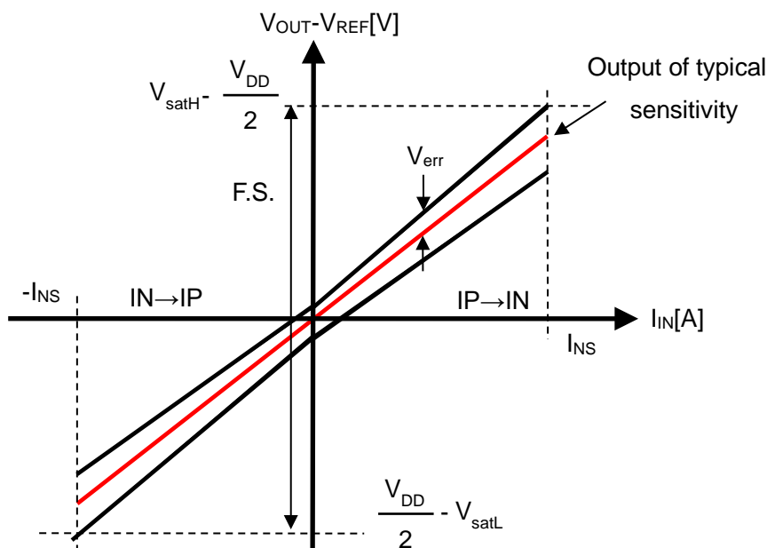
Figure 4. Total Accuracy of CZ-375B
