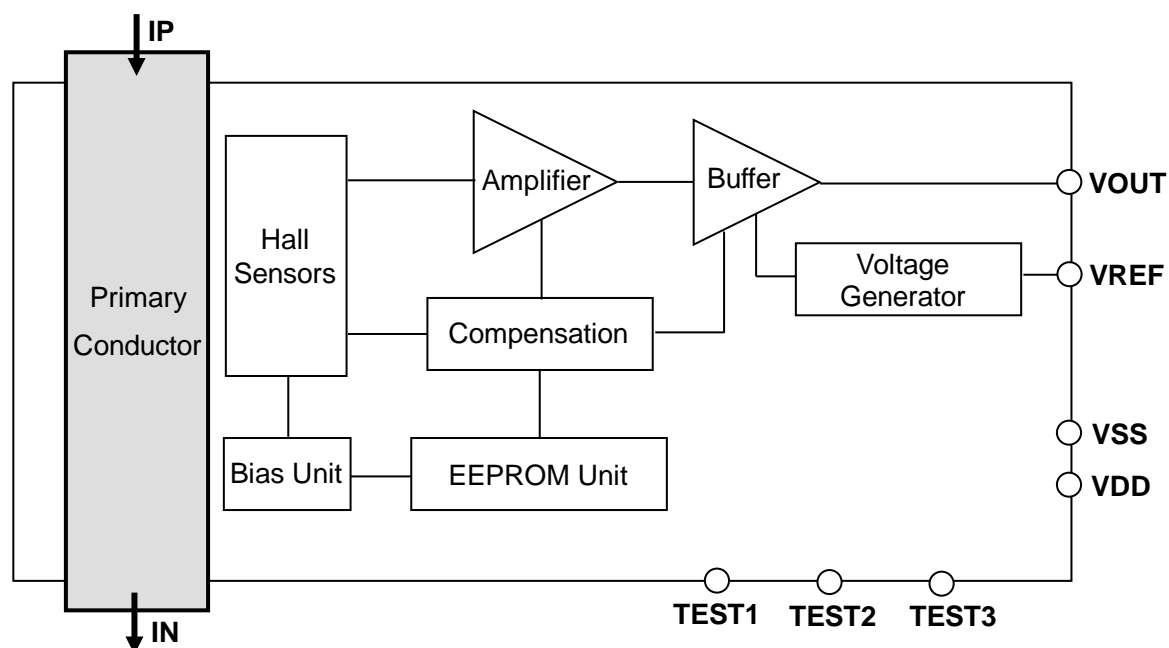
Figure 1. Block diagram of CZ-375B
