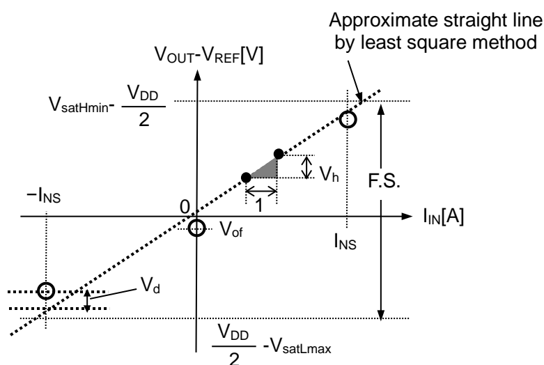
Figure 3. Characteristic definitions of CZ-375B
