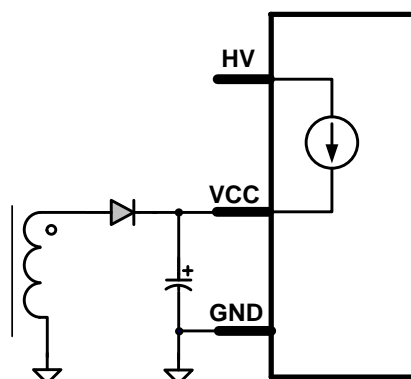
Figure 13: Start-up Circuit
