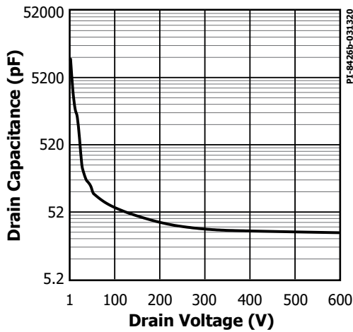
Figure 20. C_{oss} vs. Drain Voltage (INN3977CQ).
