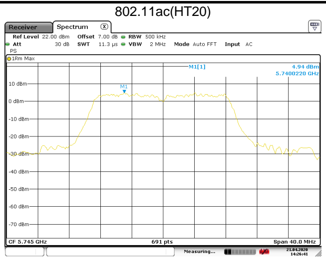
Middle channel
