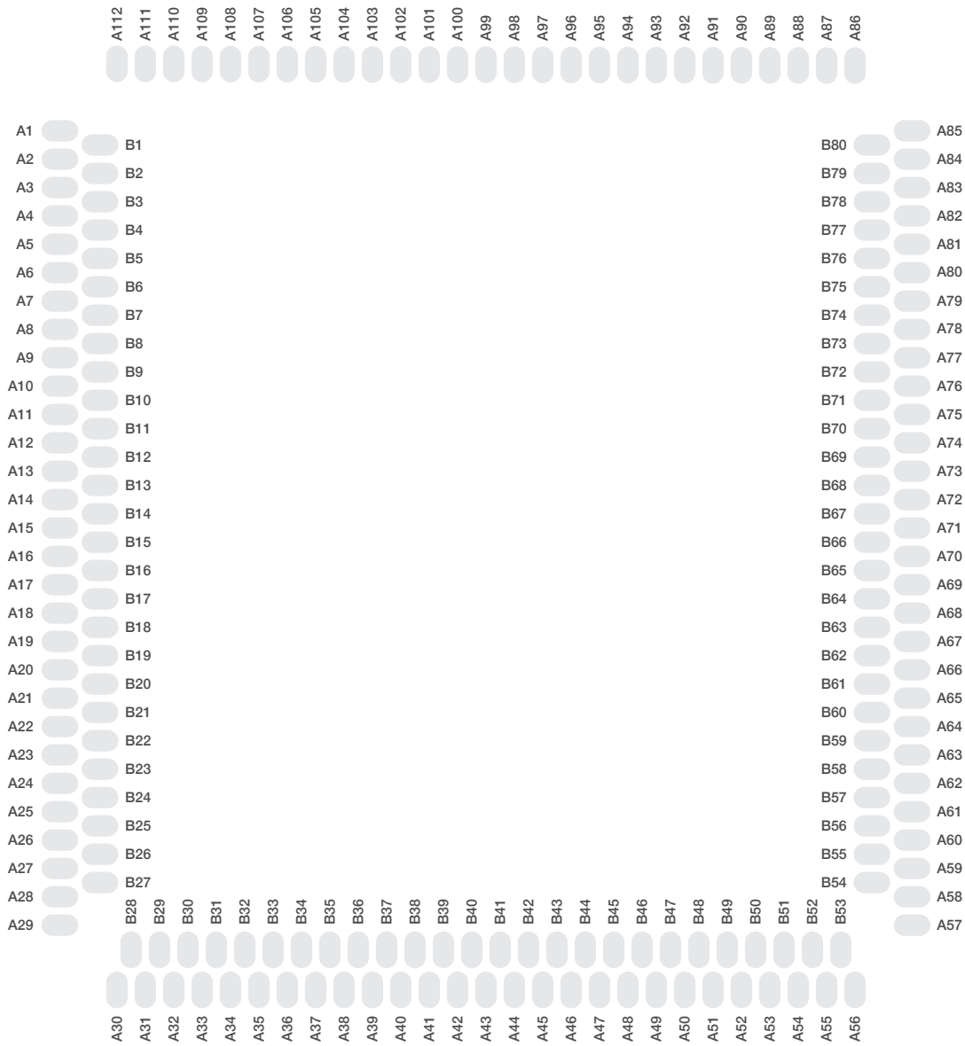
FIGURE 3-1. PIN ASSIGNMENTS
