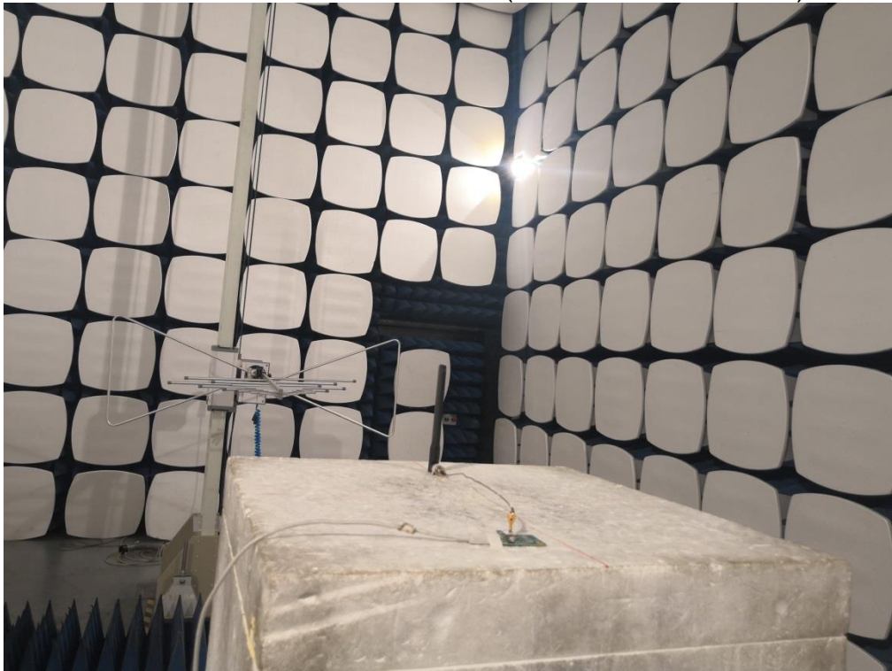
Radiated Emission Below 1GHz (for External antenna A)
