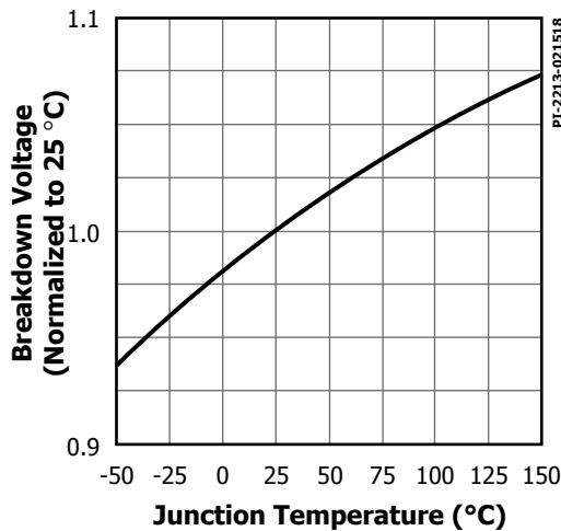
Figure 32. Breakdown vs. Temperature (Exclude INN3679C/INN3670C).
