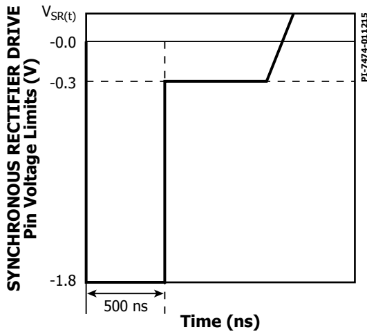
Figure 26. SYNCHRONOUS RECTIFIER DRIVE Pin Negative Voltage.
