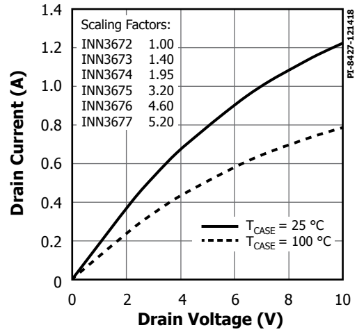
Figure 23. Output Characteristics.
