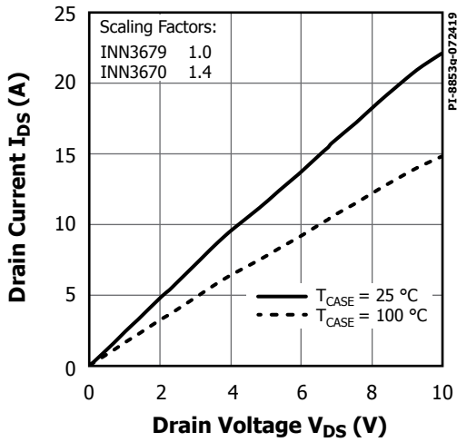
Figure 33. Output Characteristics.
