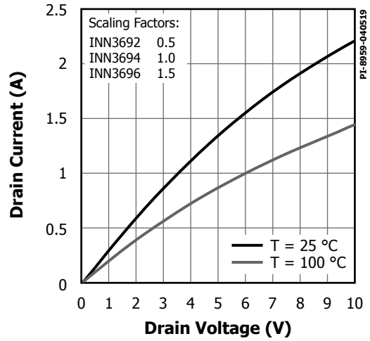
Figure 29. Output Characteristics.
