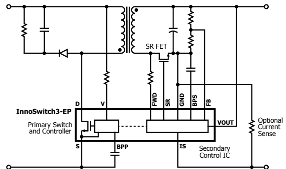
Figure 1. Typical Application Schematic.
