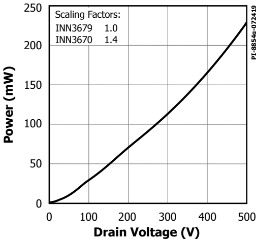
Figure 35. Drain Capacitance Power.
