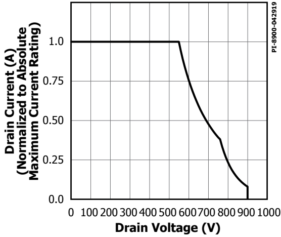
Figure 28. Maximum Allowable Drain Current vs. Drain Voltage (INN369x).
