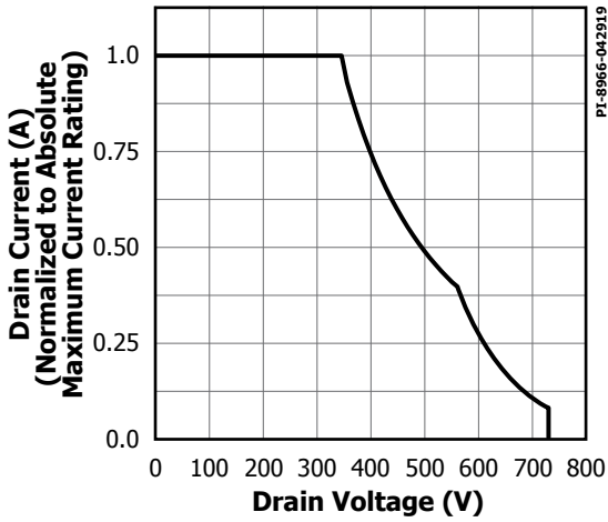
Figure 22. Maximum Allowable Drain Current vs. Drain Voltage (INN3672-INN3677).
