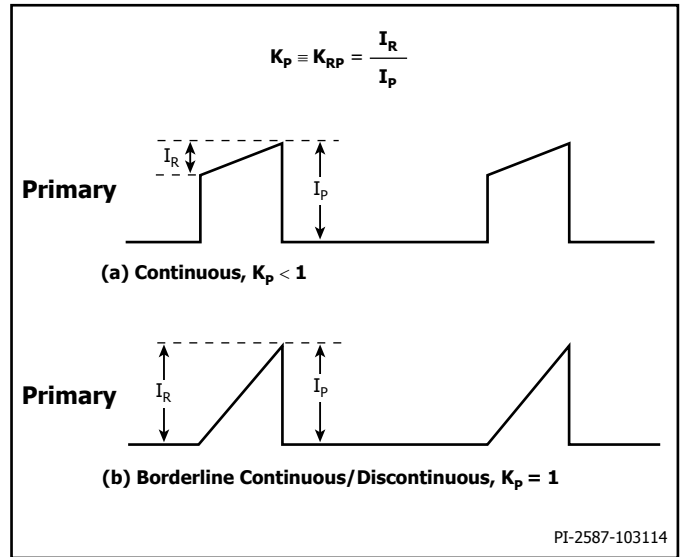
Figure 18. Continuous Conduction Mode Current Waveform, K_p < 1 .
