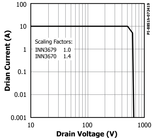
Figure 36. Maximum Allowable Drain Current vs. Drain Voltage (GaN-based INN3679-INN3670).
