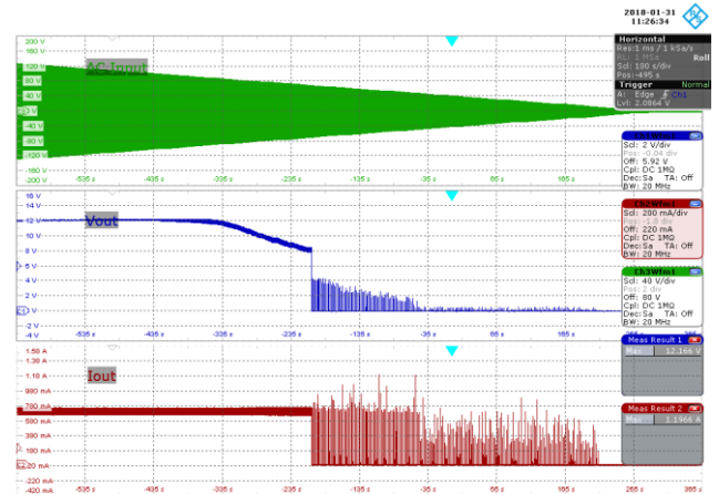
Figure 93 – Brown-out Test. 90 to 0 VAC at 0.1 V / s. CH1: V_{OUT} , 2 V / div., 100 s / div. CH2: I_{OUT} , 200 mA / div., 100 s / div. CH3: AC_{IN} , 40 V / div., 100 s / div. Highest Average Input Power: 10.575 W at 64.2 VAC.
