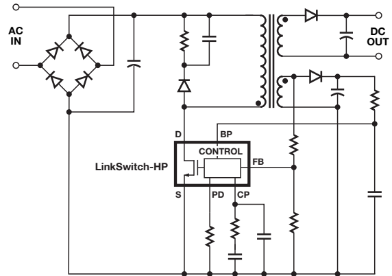
Figure 1. Typical Application Schematic.
