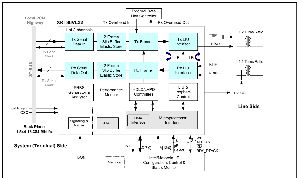
FIGURE 1. XRT86VL32 2-CHANNEL DS1 (T1/E1/J1) FRAMER/LIU COMBO
