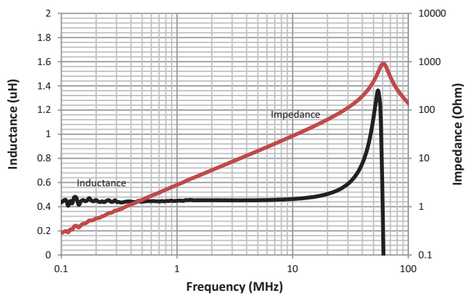
HCM1A1307V2-R47-R
