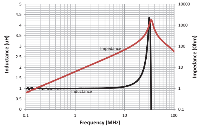
HCM1A1307V2-1R0-R
