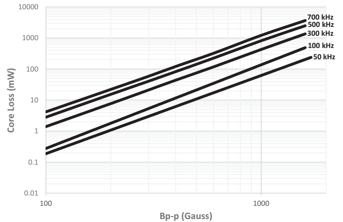
HCM1A1307V2-6R8-R
