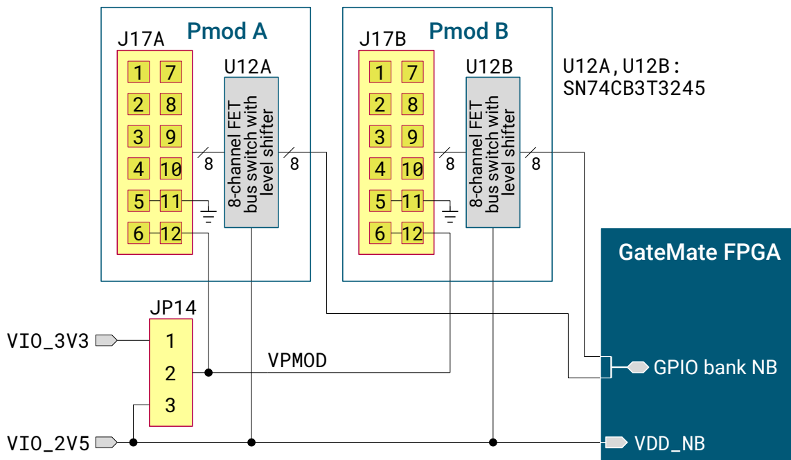
Figure 3.17: GPIO bank NB with Pmod interface
