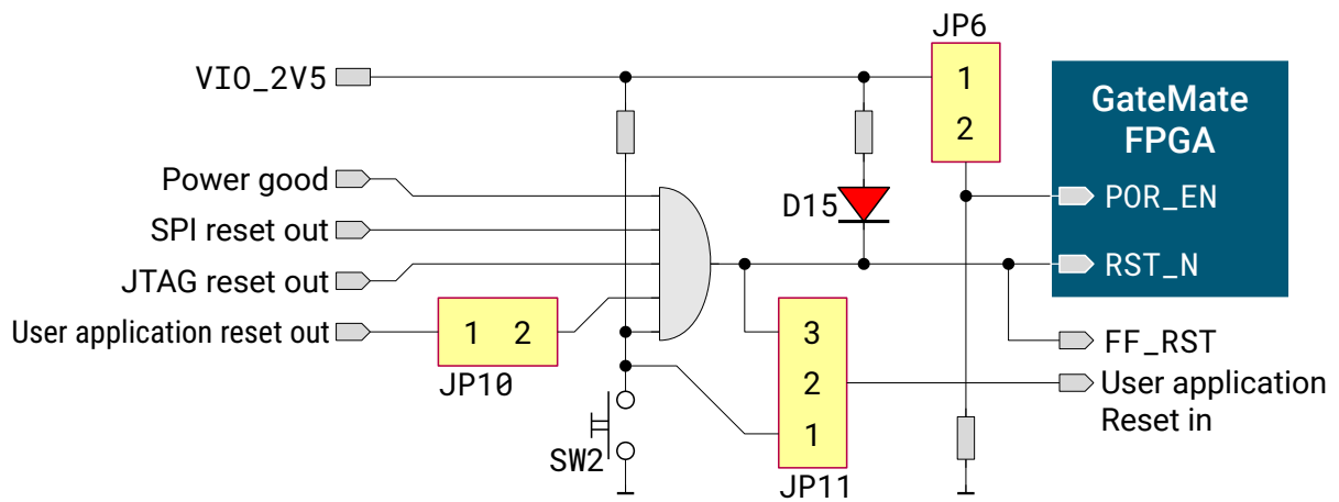
Figure 3.10: Reset module
