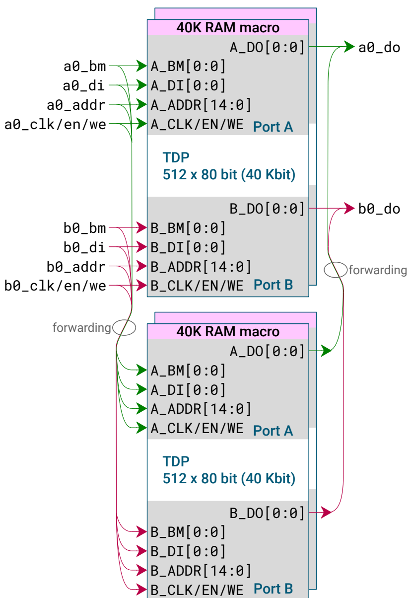
Figure 2.15: Structure of two adjacent DPSRAMs forming one 64K × 1 bit memory via cascade feature
