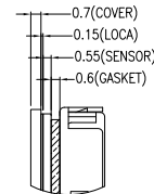
DETAIL C (SCALE 3:1)
