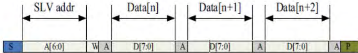
Figure 1-2 IIC Master Write, Slave Red
