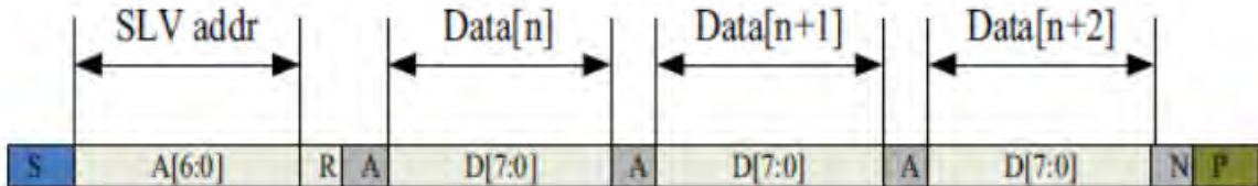
Figure 1-3 IIC Master Red, Slave Write
