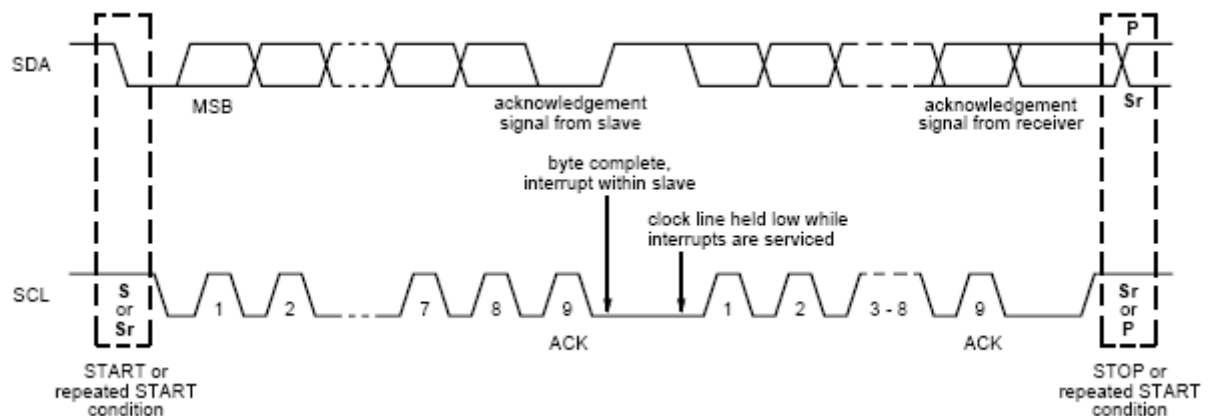
Figure 1-1 IIC Serial Data Transfer Format
