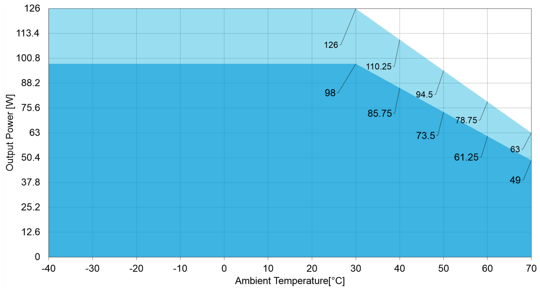
Figure 5. Power Derating of 12 V & 15 V models (Cove kit option)
