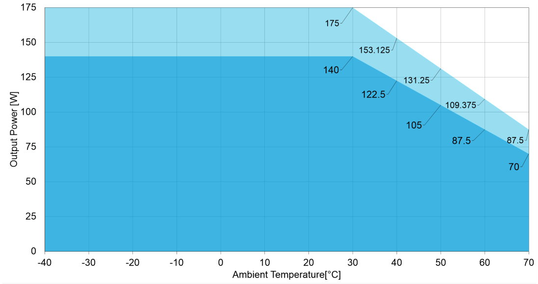
Figure 4. Power Derating of 24 V, 30 V, 48 V & 58 V models (Cove kit option)
