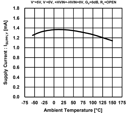
Supply Current vs. Temperature (Common to each ver) V^+=5V , V=0V , +HVIN=-HVIN=0V , G_V=0dB , R_L=OPEN
