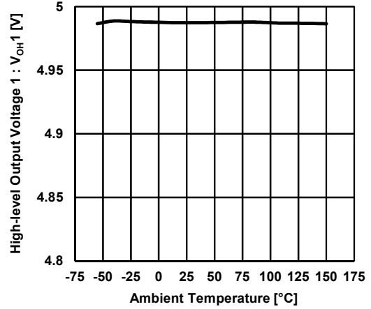
High-level Output Voltage 1 vs. Temperature (Common to each ver) V^+=5V , V=0V , R_L=10k\Omega to 2.5V
