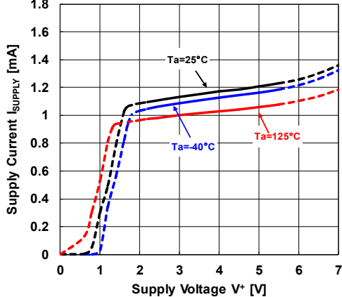
Supply Current vs. Supply Voltage (Common to each ver) V^+=5V , V=0V , +HVIN=-HVIN=0V , G_V=0dB , R_L=OPEN
