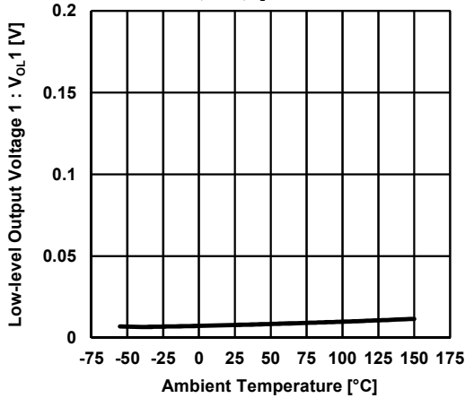
Low-level Output Voltage 1 vs. Temperature (Common to each ver) V^+=5V , V=0V , R_L=10k\Omega to 2.5V
