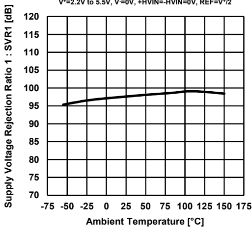
Supply Voltage Rejection Ratio 1 vs. Temperature (Common to each ver) V^+=2.2V to 5.5V , V=0V , +HVIN=-HVIN=0V , REF=V^+/2
