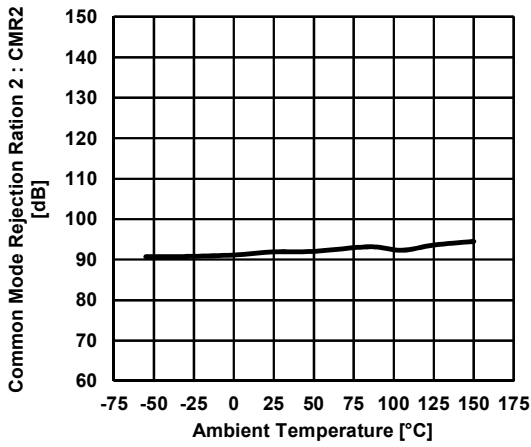
Common Mode Rejection Ratio 2 vs. Temperature V^+=5V, V^-=0V, +OPIN=0V to 4V
