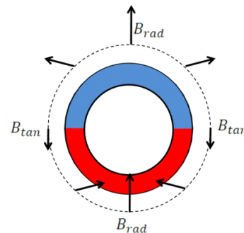
Figure 20: Side-Shaft Field
