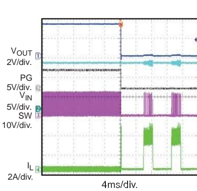
SCP Entry I_{OUT}=0A
