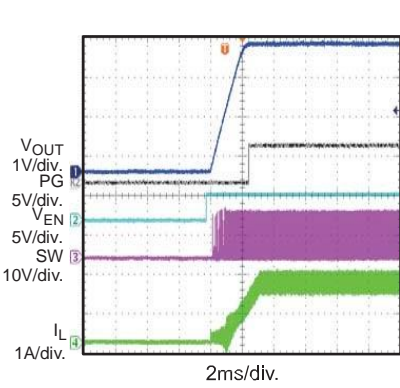
Start-Up through EN/SYNC I_{OUT}=1.5A
