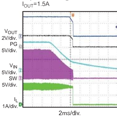
Shutdown through Input Voltage I_{OUT}=1.5A
