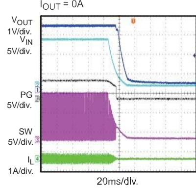
Shutdown through Input Voltage I_{OUT}=0A
