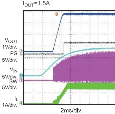
Start-Up through Input Voltage I_{OUT}=1.5A
