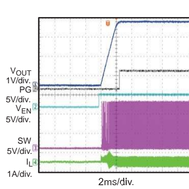
Start-Up through EN/SYNC I_{OUT}=0A
