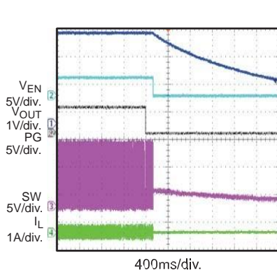
Shutdown through EN/SYNC I_{OUT}=0A
