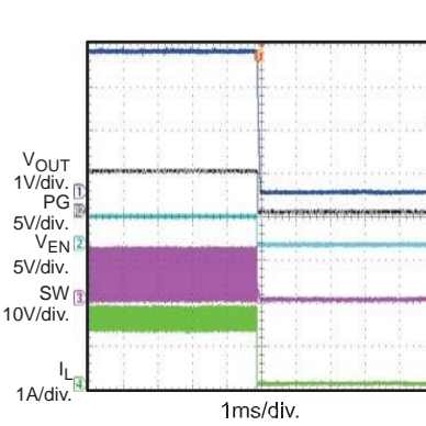
Shutdown through EN/SYNC I_{OUT}=1.5A
