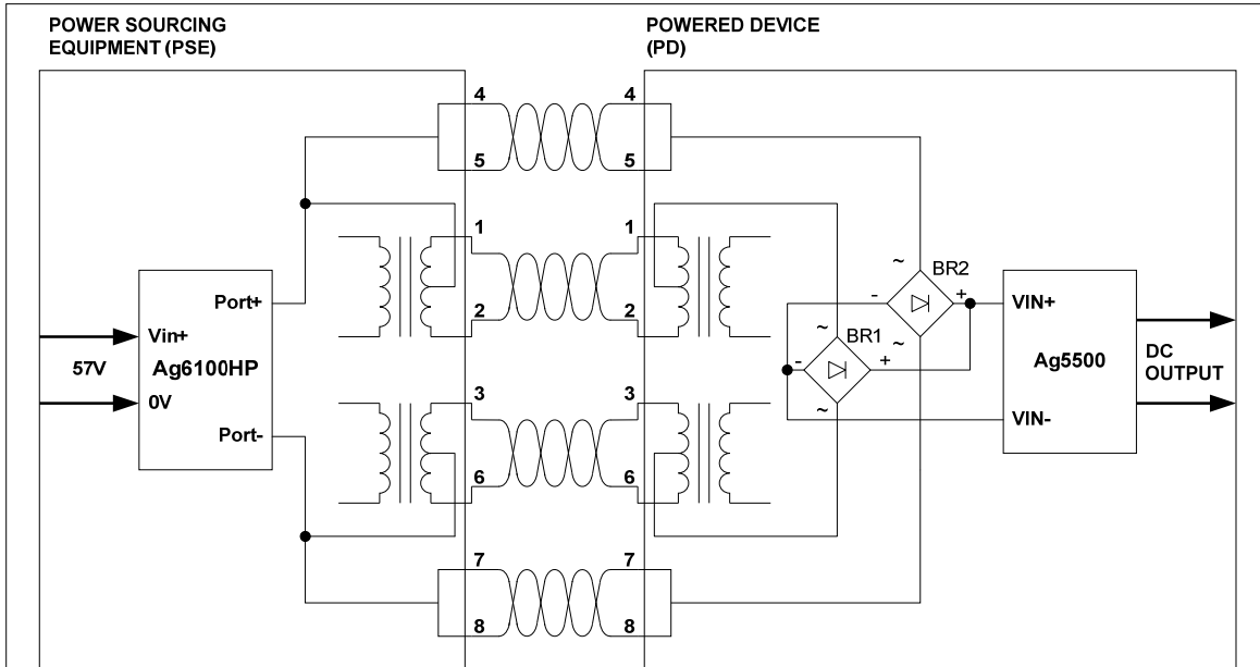
Figure 8a – Typical Application Diagram for Ag6100-HP using 10/100BASE-T
