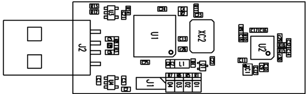
Figure 2-3 Assembly drawing RZRAVEN - front view.
