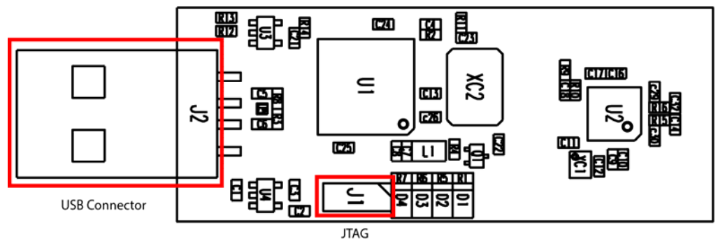
Figure 4-1 RZRAVEN Interfaces - front.
