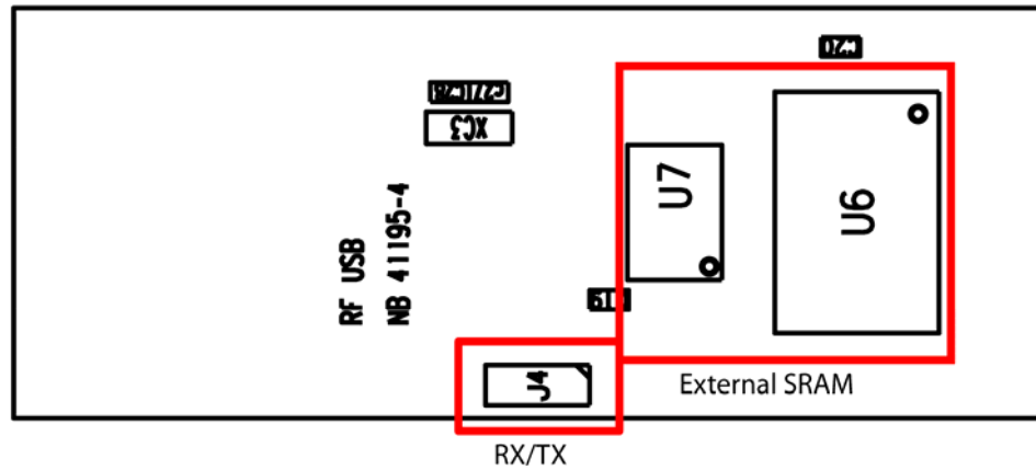
Figure 4-2 RZRAVEN Interfaces - back
