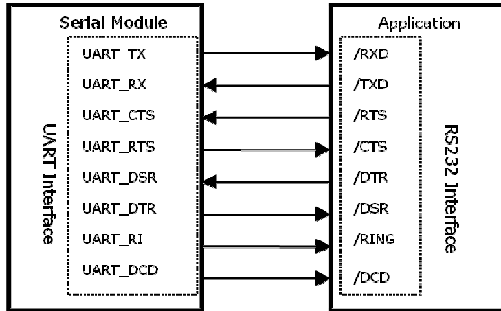
Figure 6.1 : UART interfaces
