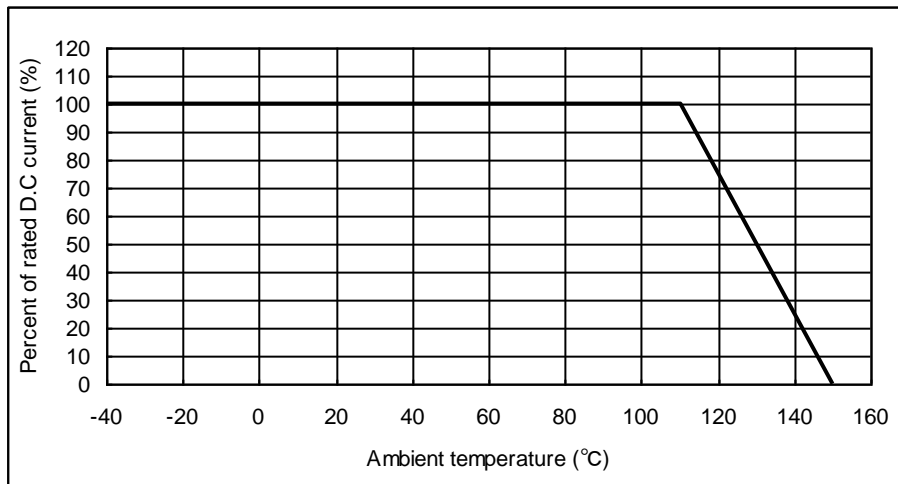
Derating Curve
